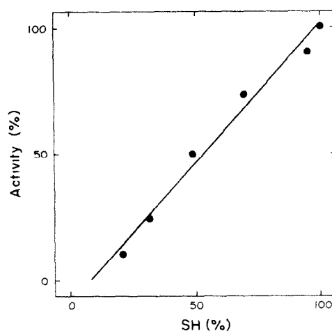
Fig. 2. Proportionality of activity and thiol content of papain as percentage of initial values, during inactivation of the enzyme by DIMBOA. Initial specific activity was 8.9 \mu\text{mol/min/mg} protein, and initial thiol titre was 0.57 \text{ mol SH/mol enzyme} .
