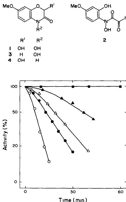
Fig. 1. Kinetics of papain inactivation at different DIMBOA concentrations. 0 (■), 3 (▲), 5 (△), 8 (●), and 15 mM (○), in 50 mM phosphate buffer, pH 6.8, at 28°. The concentration of papain was 1.1 \times 10^{-5} M. The curves represent the fit of the experimental points to eqn (1). Initial specific activity was 8.1 \mu\text{mol/min/mg protein} .
